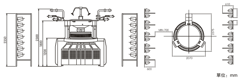
机器外观尺寸 External dimension of machine
